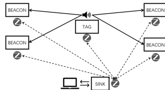
Fig. 2. Conceptual architecture of mAidLoc demo system.
