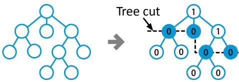
Fig. 2: Tree cut example: the cut is denoted by the dotted line. Every node above the dotted line is labeled 1, while the others are labeled 0.
