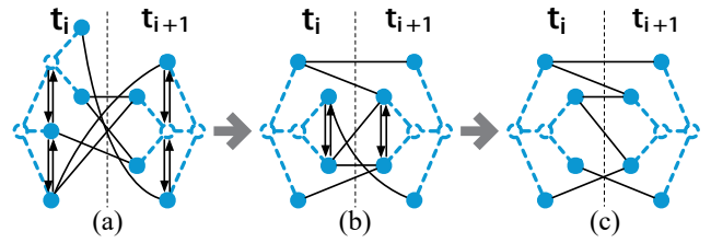
Fig. 6: Reordering example: (a) reorder level one; (b) reorder level two; (c) result.
