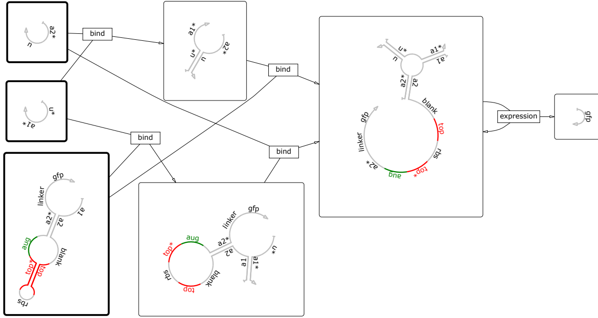
Fig. 1: Reaction network of a ribocomputing AND gate with input triggers \langle u * a1 * \rangle and \langle a2 * u \rangle . After the triggers bind to the AND gate, the ribosome binding site rbs is exposed and translation of \langle gfp \rangle is activated in a catalytic loop.
