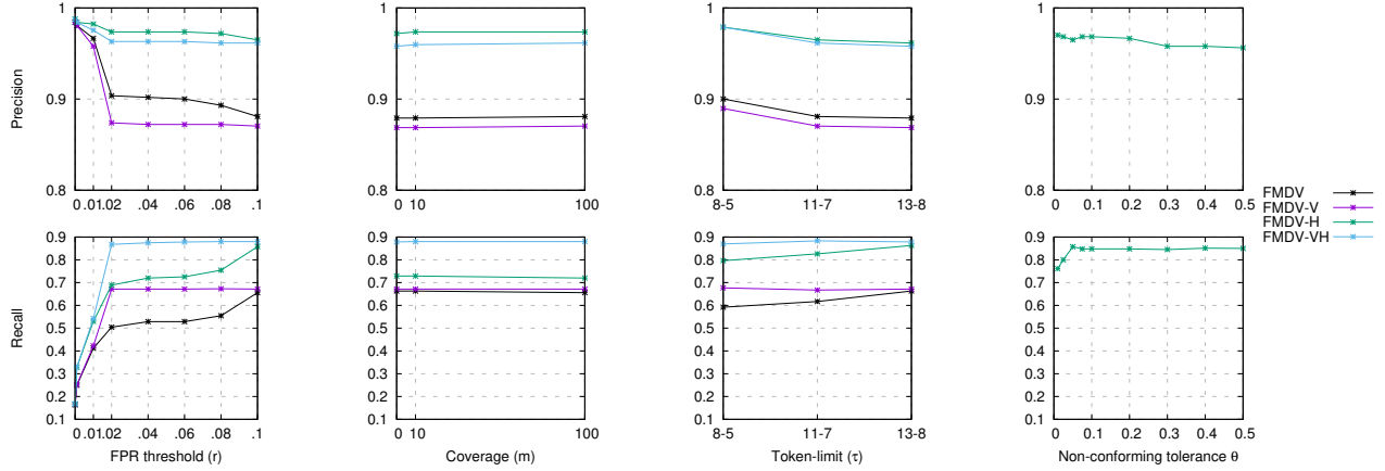
(a) Sensitivity to FPR threshold ( r ) (b) Sensitivity to Coverage ( m ) (c) Sensitivity to token-limit ( \tau ) (d) Sensitivity of FMDV-H to ( \theta )
