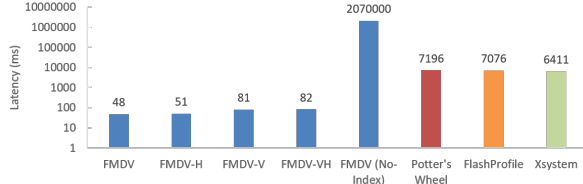
Figure 13: Latency in milliseconds (per query column).
