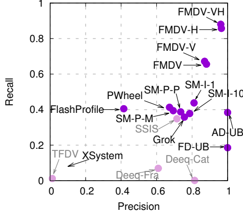
(a) Enterprise benchmark: Numbers reported using a subset of 571 cases where syntactic patterns exist.
