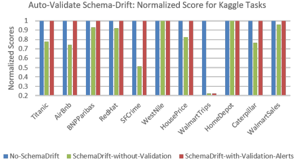
Figure 14: Impact of schema-drift on Kaggle tasks, with and without data-validation. FMDV detects drift in 8/11 cases.
