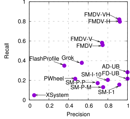
(b) Government benchmark: Numbers reported using a subset of 359 cases where syntactic patterns exist.
