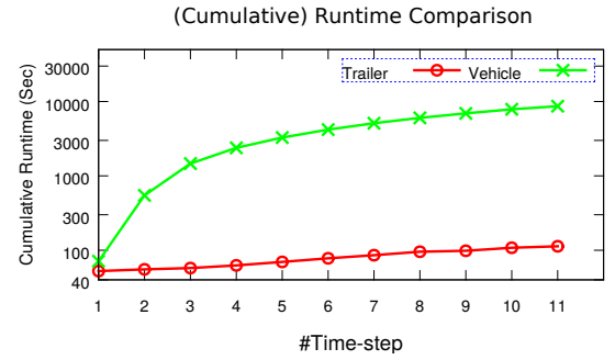
Figure 3: (Cumulative) Runtime comparison between the repositioning solutions of vehicles and trailers.
