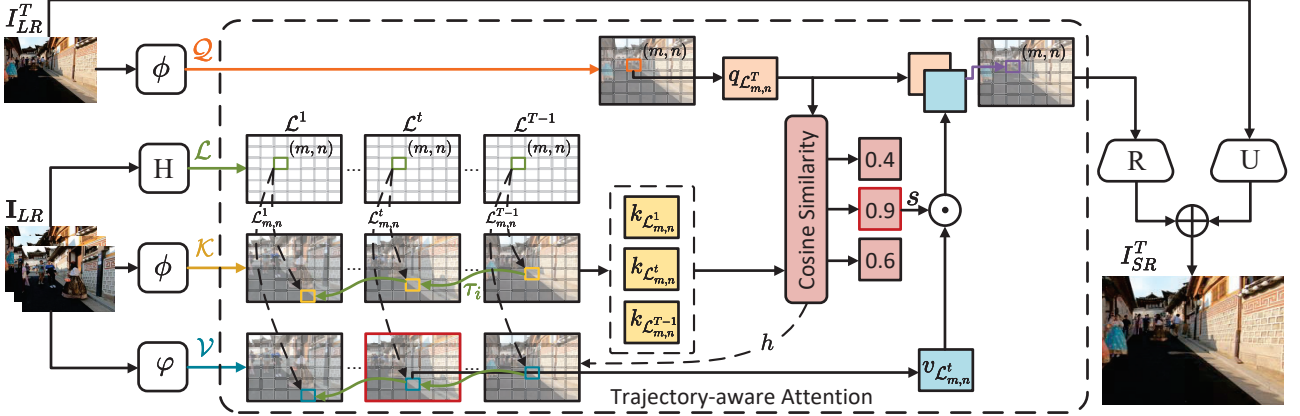
Figure 2. The overview of TTVSR based on location maps. Q , K and V are tokens from video frames extracted by embedding networks \phi(\cdot) and \varphi(\cdot) , respectively. \tau_i indicates a trajectory of \mathcal{T} . \mathcal{L} is the set of location map generated by the motion estimation network H . The dotted lines indicates the indexing operation from K and V by location maps \mathcal{L} and hard index h . R(\cdot) represents the reconstruction network followed by a pixel-shuffle layer to resize feature maps to the desired size. U(\cdot) represents the bicubic upsampling operation. \odot and \oplus indicate multiplication and element-wise addition, respectively.
