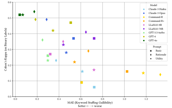
Figure 9: Cohen’s \kappa scores against the average MAE of all keyword stuffing gullibility tests for each LLM-prompt combination.
