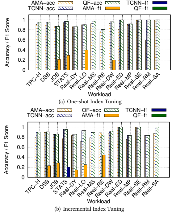
Figure 7: Comparison of ML-based regression detectors in terms of prediction accuracy and F1 score.
