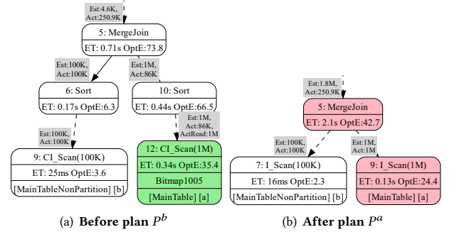
Figure 5: Illustration of regression pattern RP-3.
