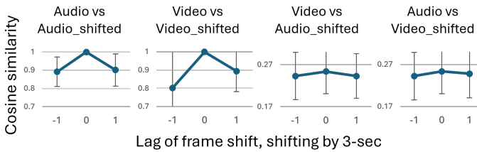
Fig. 5: Cosine similarity between AVVA embeddings as a function of audio shifts and video shifts. The data points show mean similarity scores at each shift level, comparing audio embeddings against shifted audio (panel 1) and shifted video (panel 4); and vice versa, similarity of video embeddings against shifted video (panel 2) and shifted audio (panel 3).
