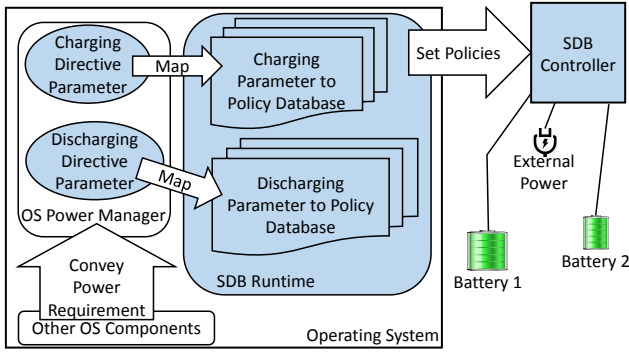
Figure 5. SDB software architecture
